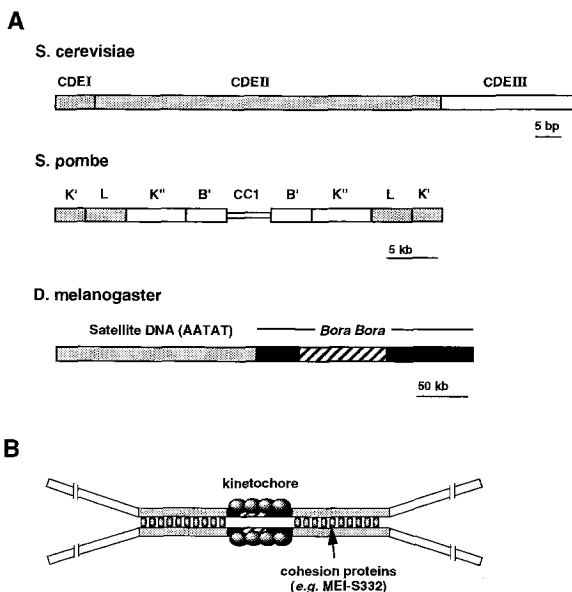
Figure 2. Centromeric Sequences Required for Sister Chromatid Cohesion
